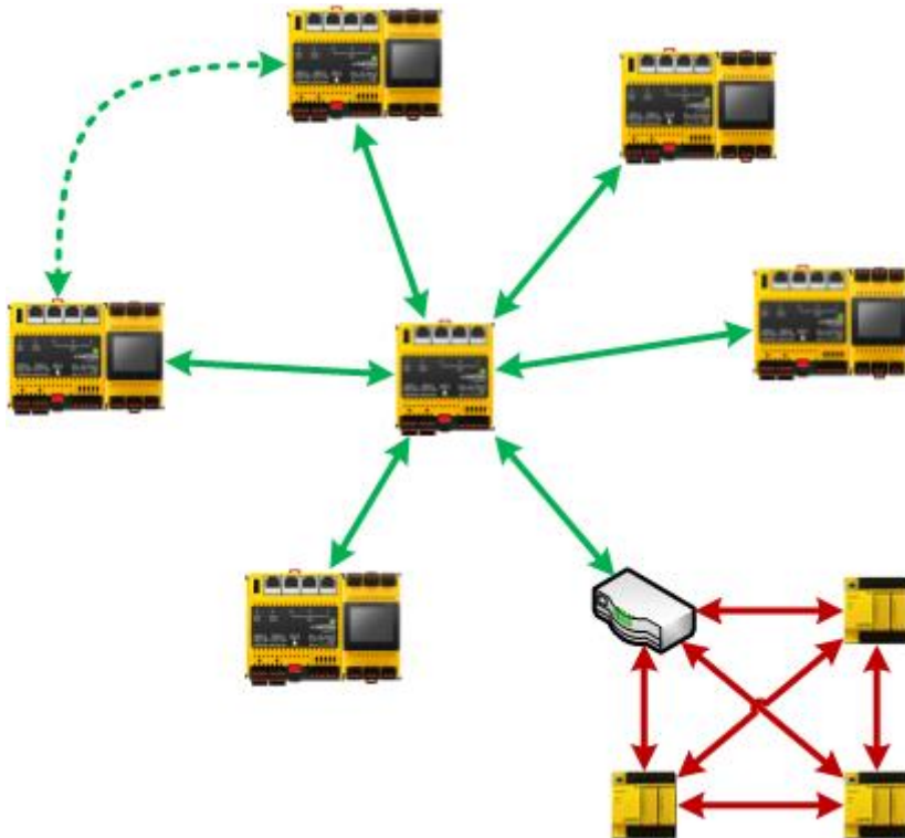
Figure 4 Hub and spoke topology of BACnet/SC. While the BACnet/SC communication is centralised in the hub, the BACnet/IP communication is station-to-station or broadcast.
