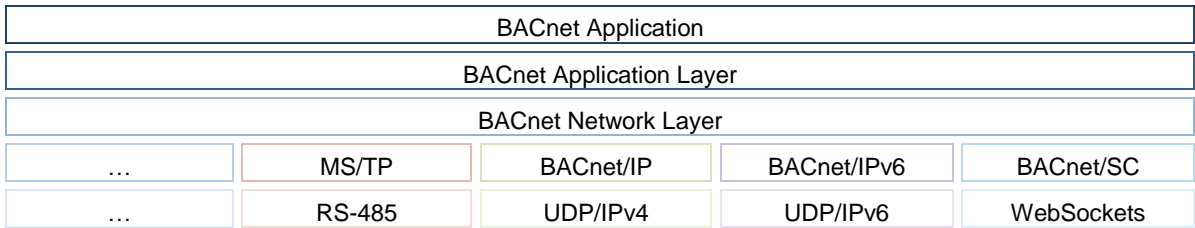
Figure 5 Representation of the different BACnet layers in the OSI layer model
