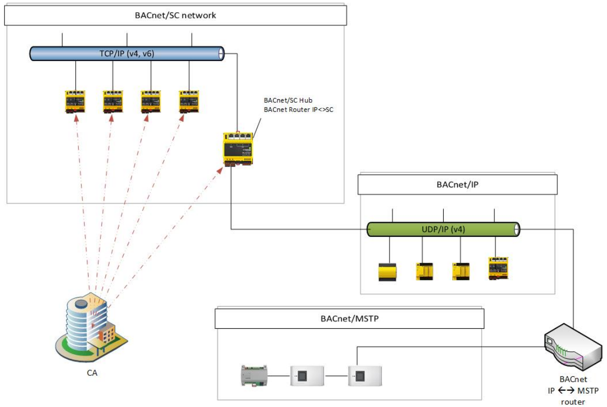
Figure 3 Various BACnet networks and devices
