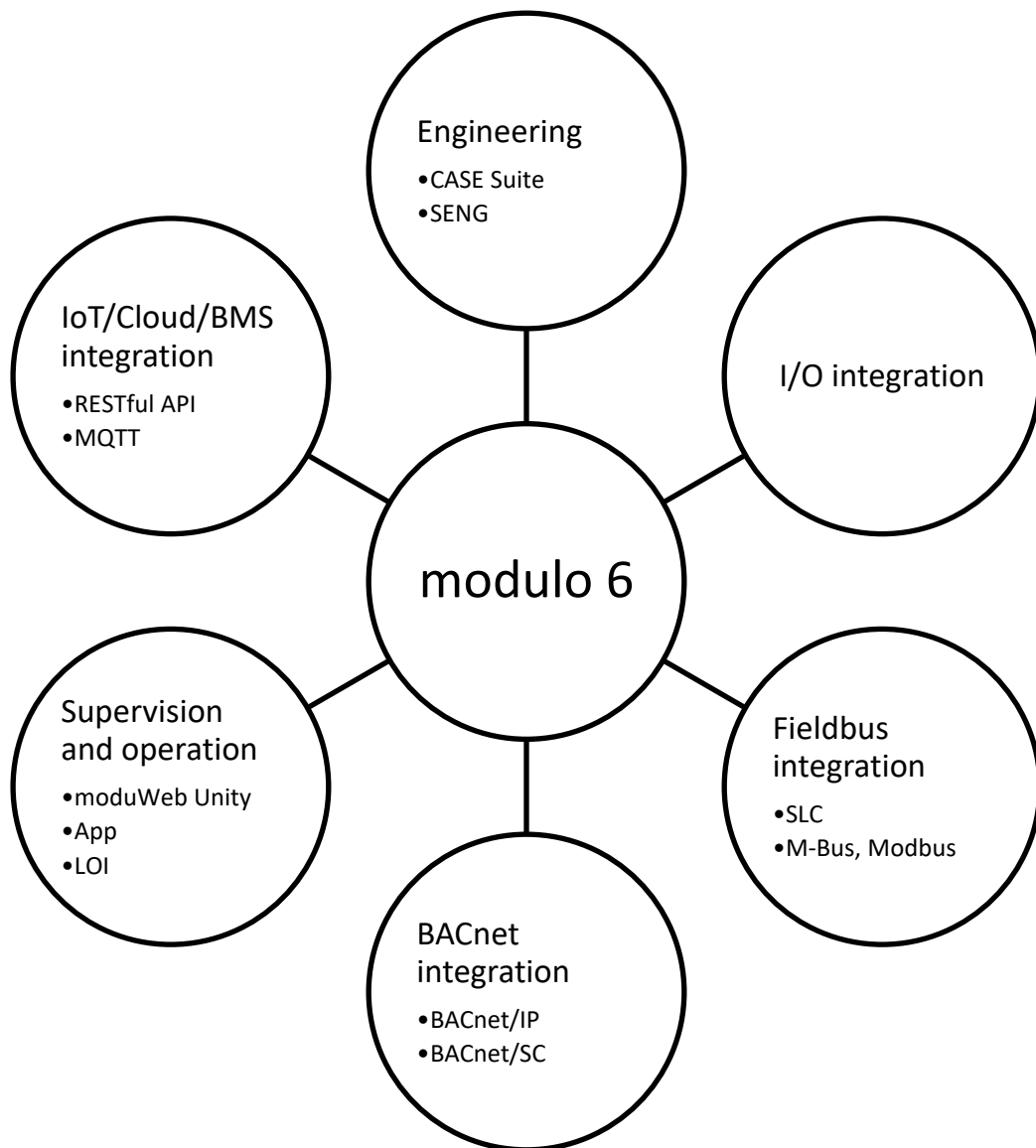
Figure 1 modulo 6 connectivity.
