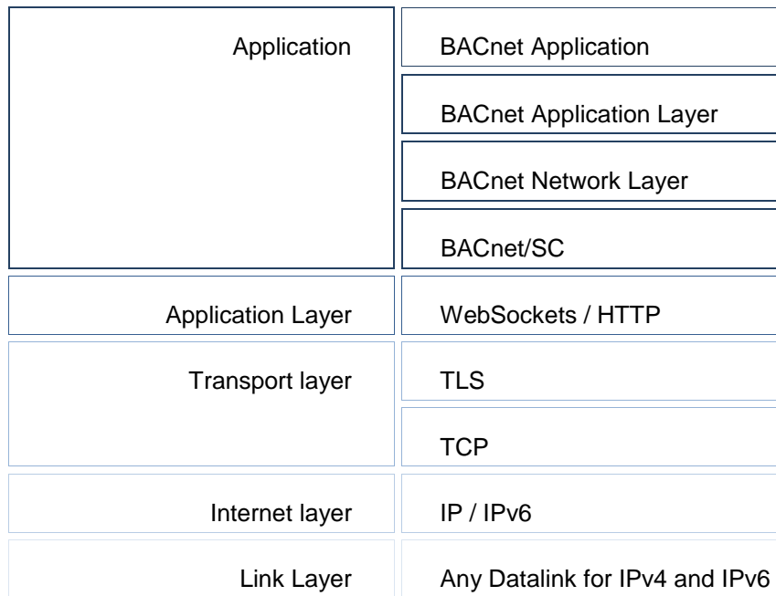
Figure 6 Representation of the BACnet/SC layers and the OSI layer model.
